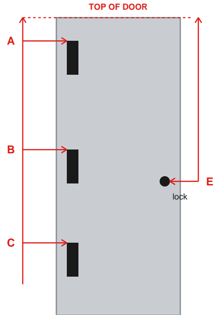
Measure top-of-door to TOP of each hinge D = 4th hinge (8' 0" doors)
