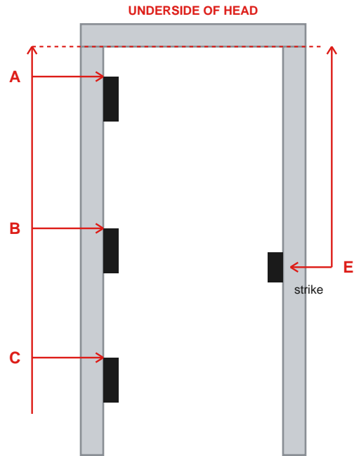
Measure underside-of-head to TOP of each hinge D = 4th hinge (8' 0" frames)
